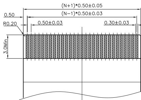
RECOMMENDED FPC/FFC DIMENSION
